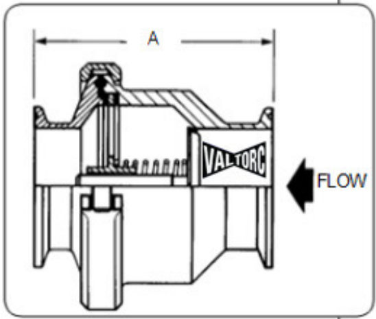
540-SN Standard Disc Type Check Valve (3A)
