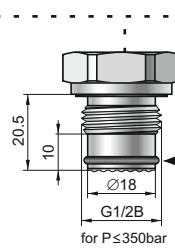
CG1/2 type G1/2" with flush diaphragm
